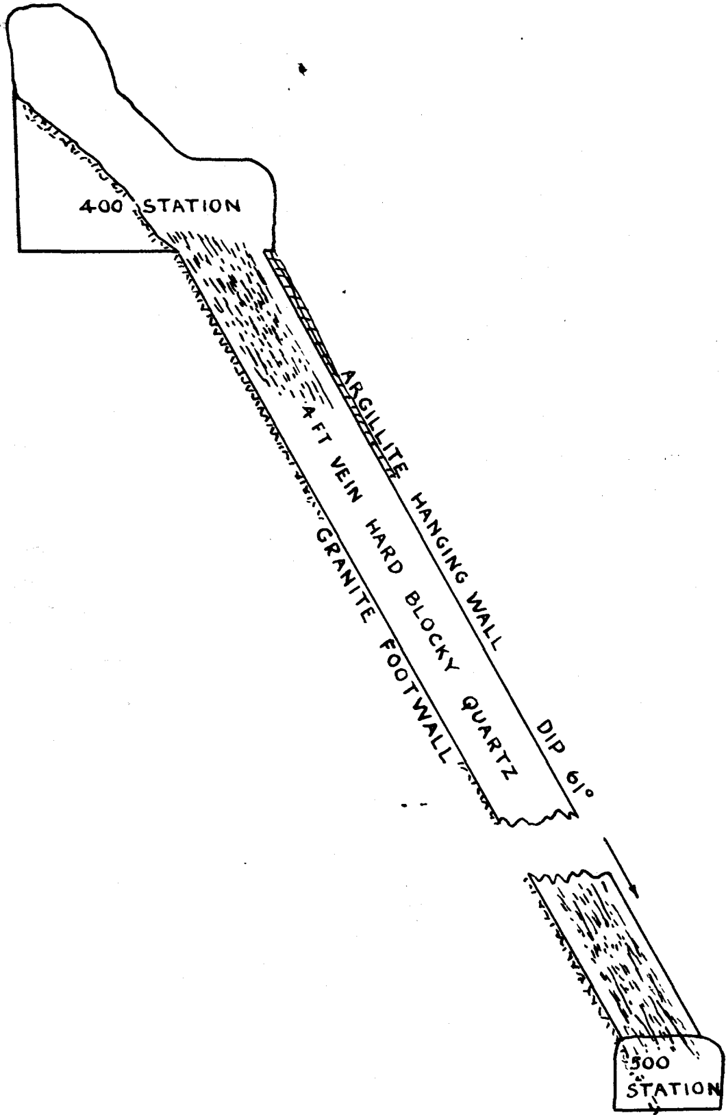
SKETCH SECTION OF 375 WINZE
