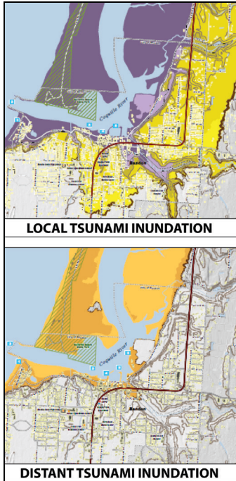
Portions of DOGAMI TIM-Coos-16, Bandon maps, showing modeled tsunami inundation for downtown Bandon and Bullards Beach.
